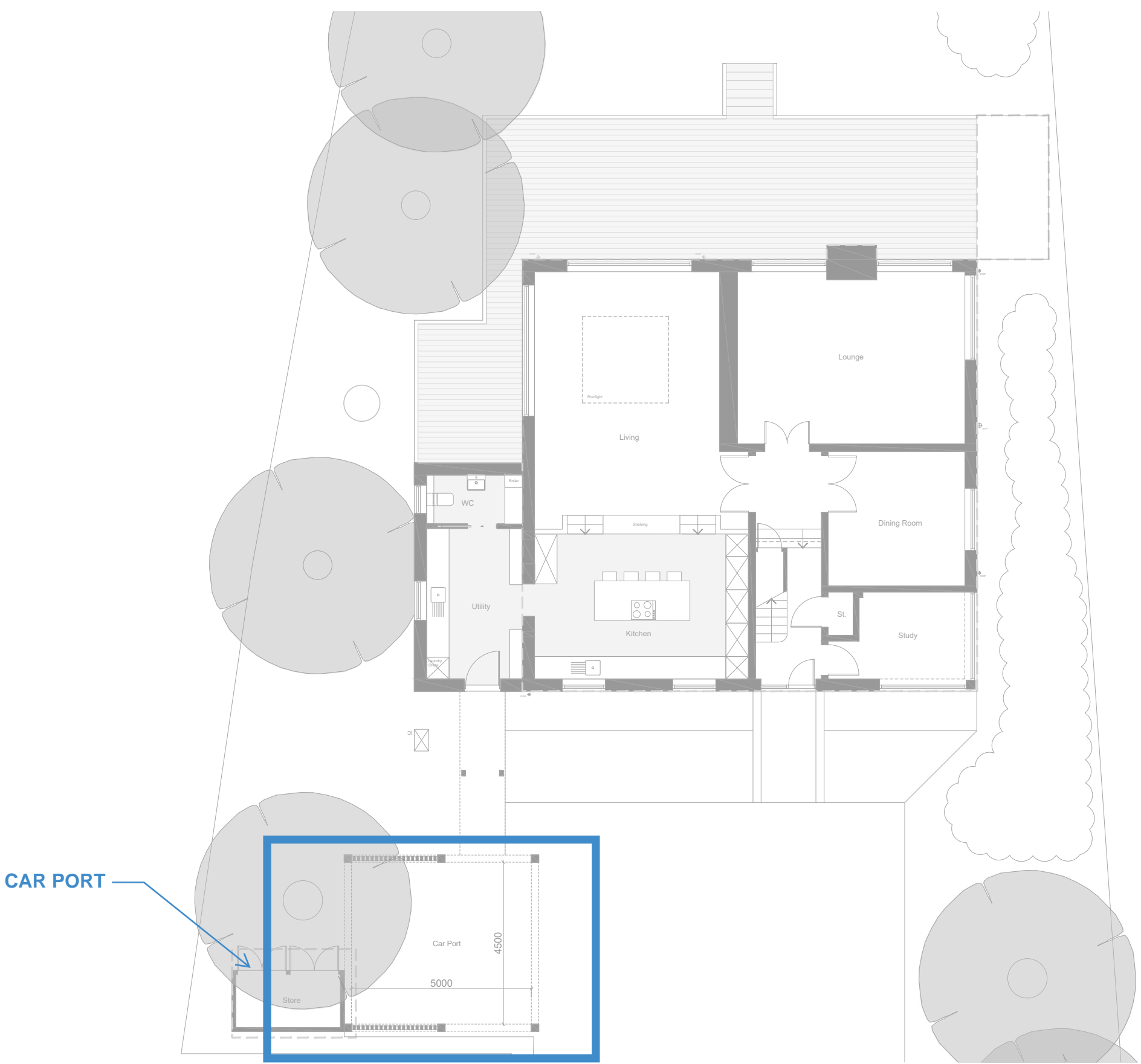
SITE PLAN
