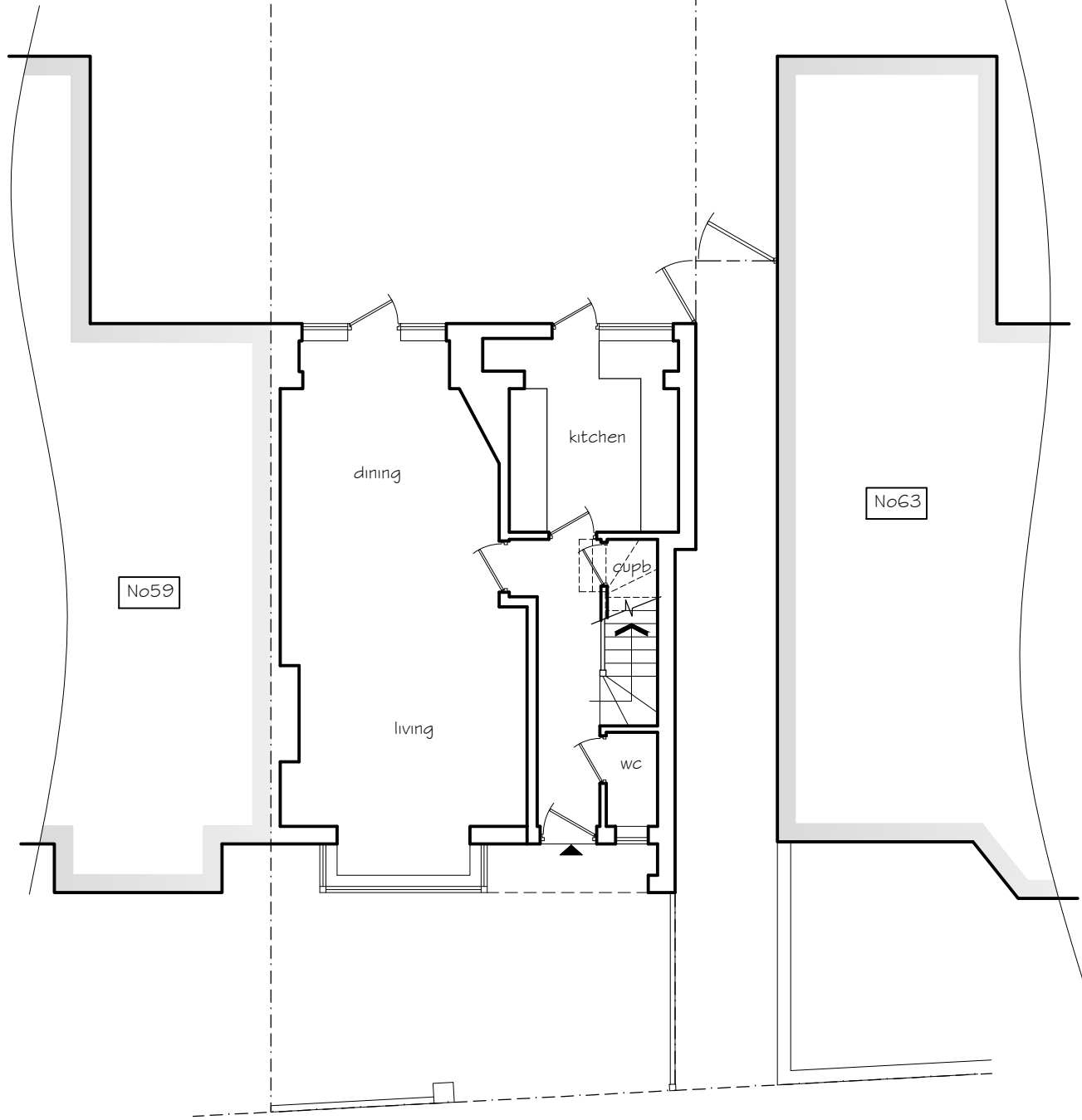
Ground Floor Plan [existing 1:100]
