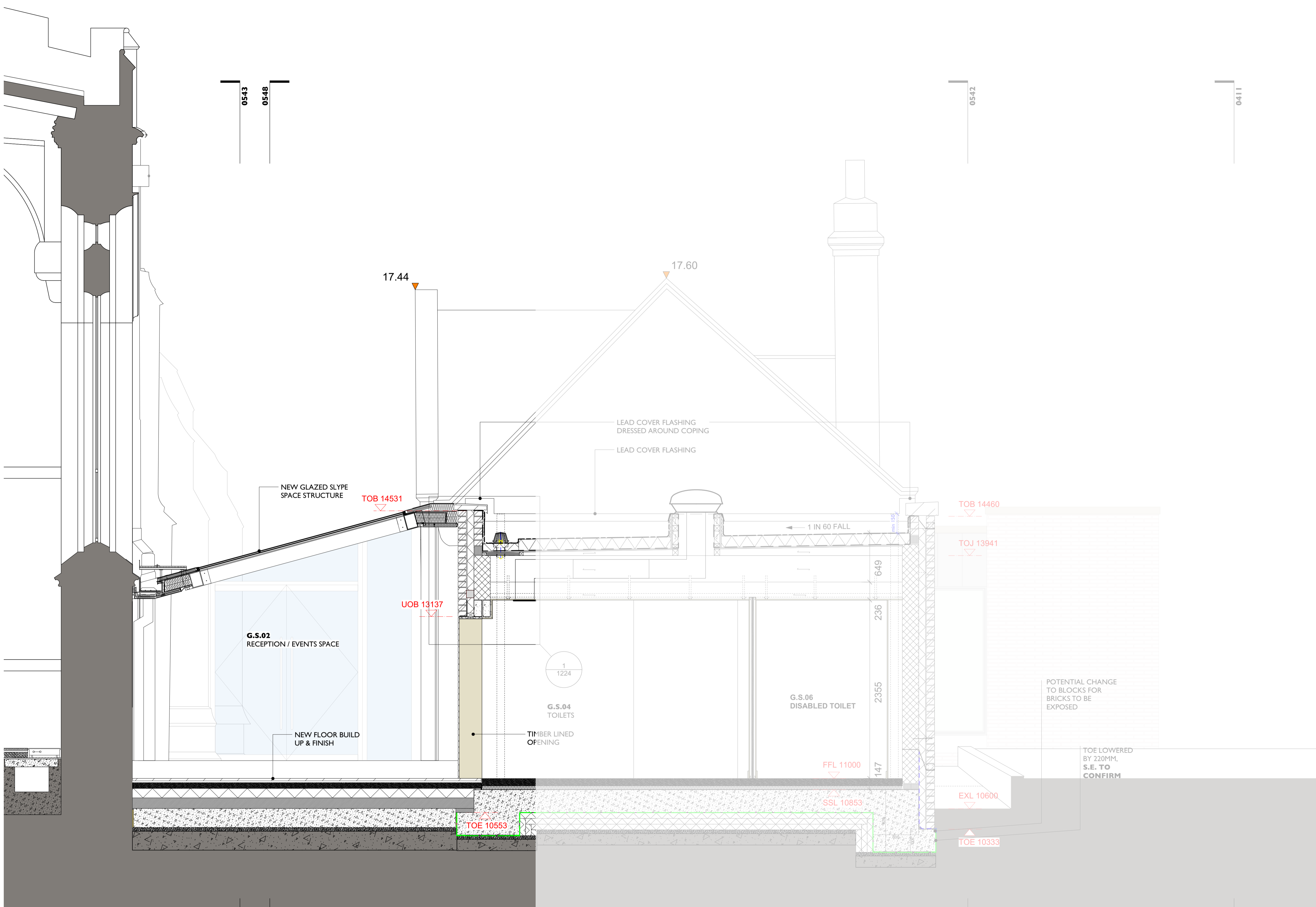
South Range Transverse Section 5 Scale: 1:25
