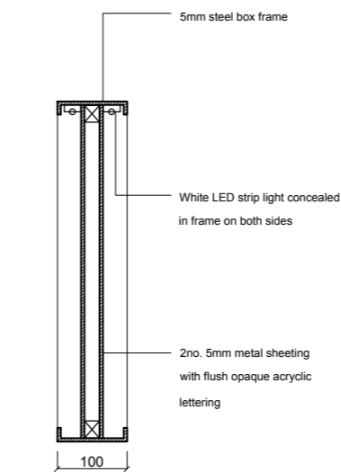
PROJECTING SIGNAGE - PROPOSED 1:10
