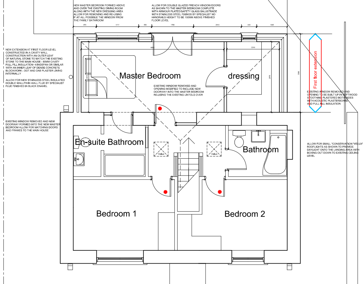
First floor plan proposed
