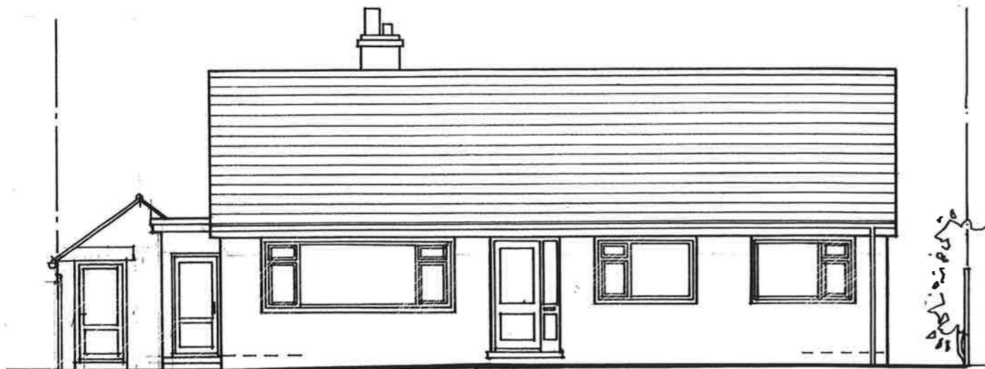
Existing South East Elevation
