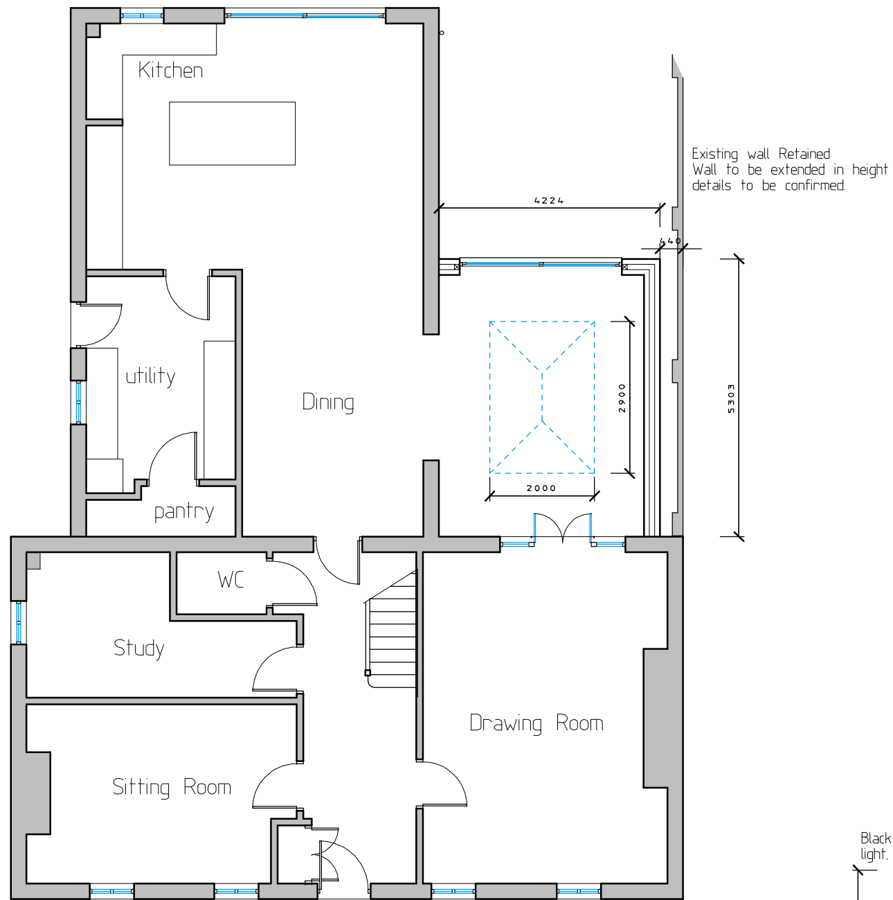
Ground Floor 1-100
