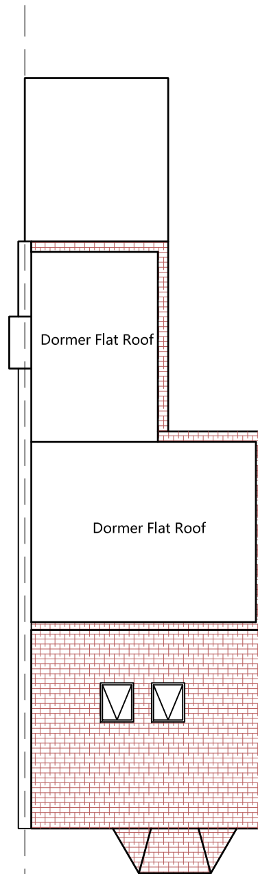
Roof Plan No Change Proposed
