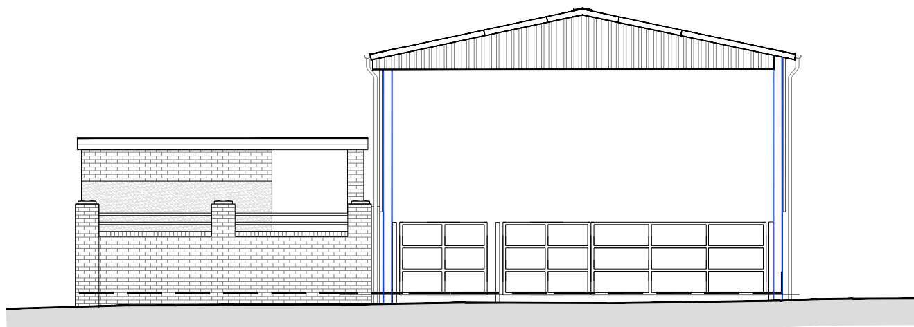
NORTH ELEVATION
