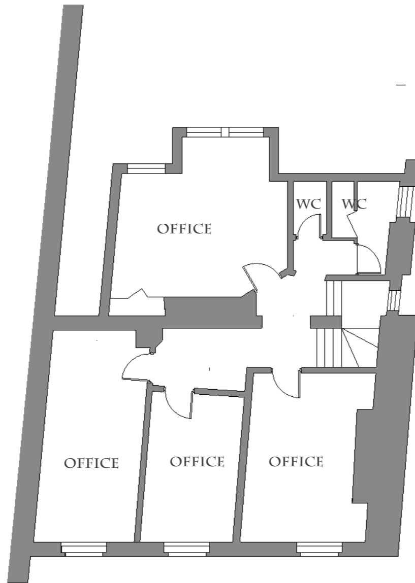
A 4 First Floor 1:100
