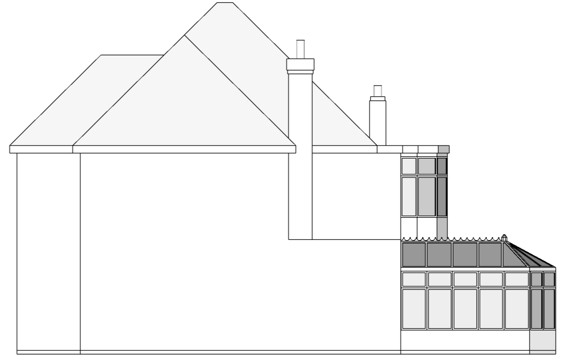
Existing RHS Elevation 1:100@A3
