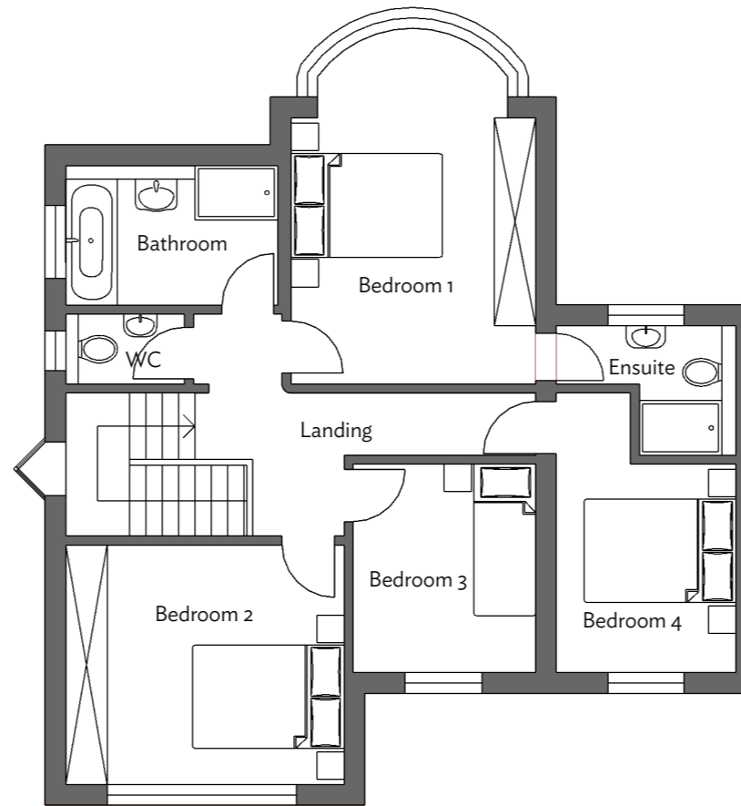
Proposed First Floor Plan 1:100@A3
