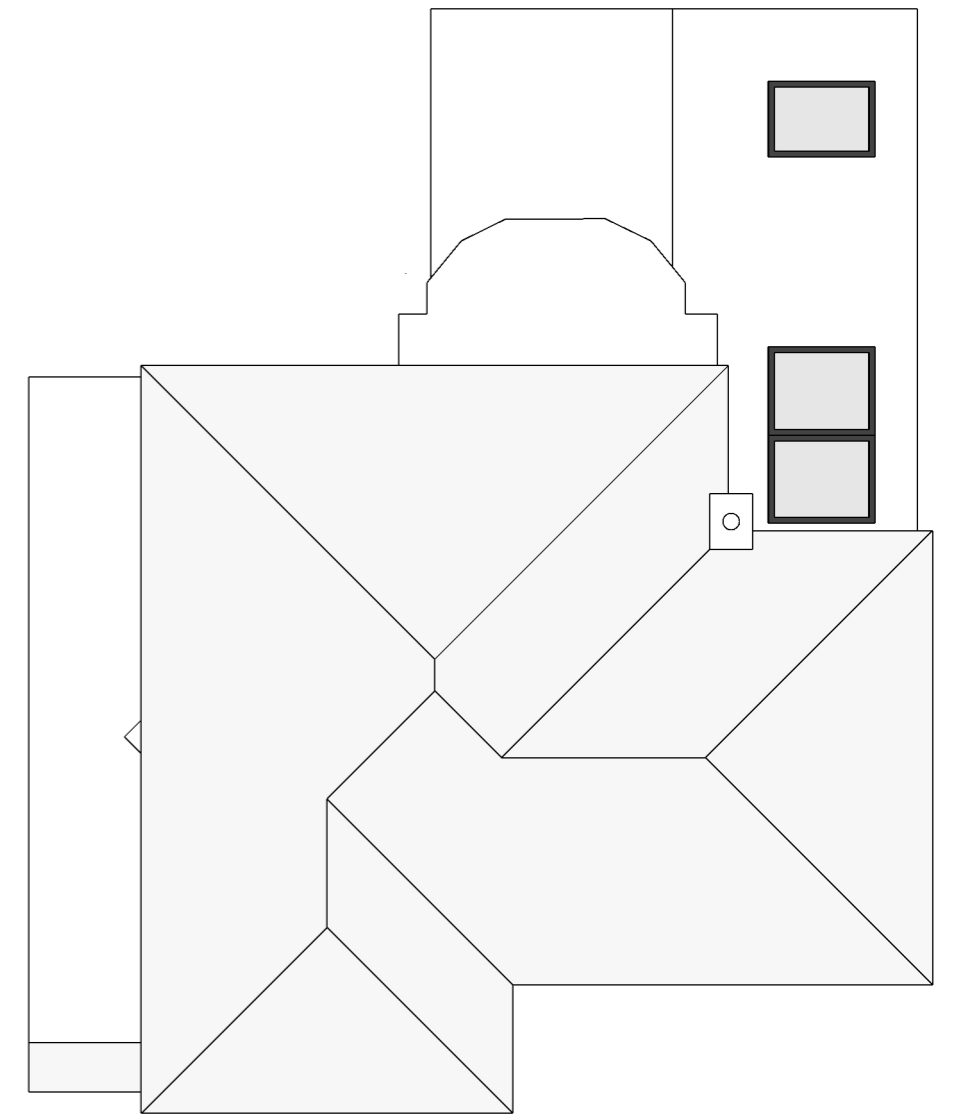
Proposed Roof Plan 1:100@A3
