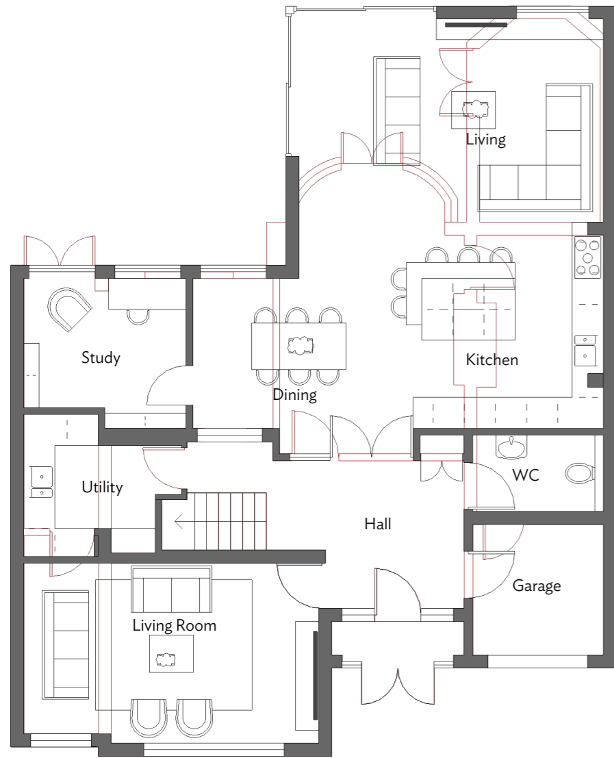
Proposed Ground Floor Plan 1:100@A3
