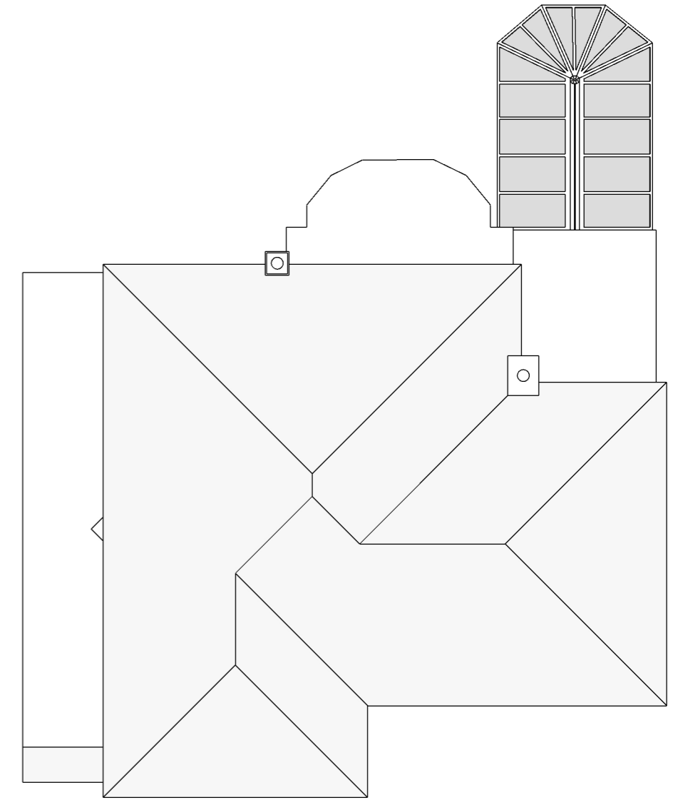
Existing Roof Plan 1:100@A3
