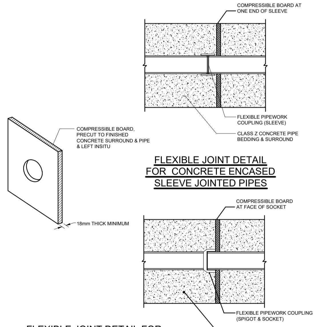
FLEXIBLE JOINT DETAIL FOR CONCRETE ENCASED PIPES (TO B.S. 1142)
