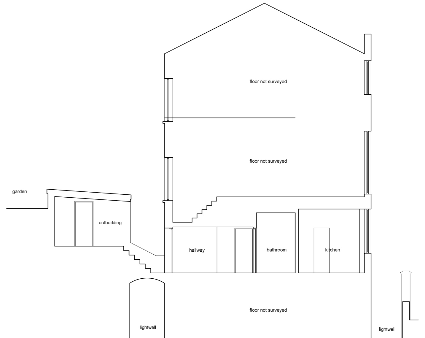
110.3 SECTION
