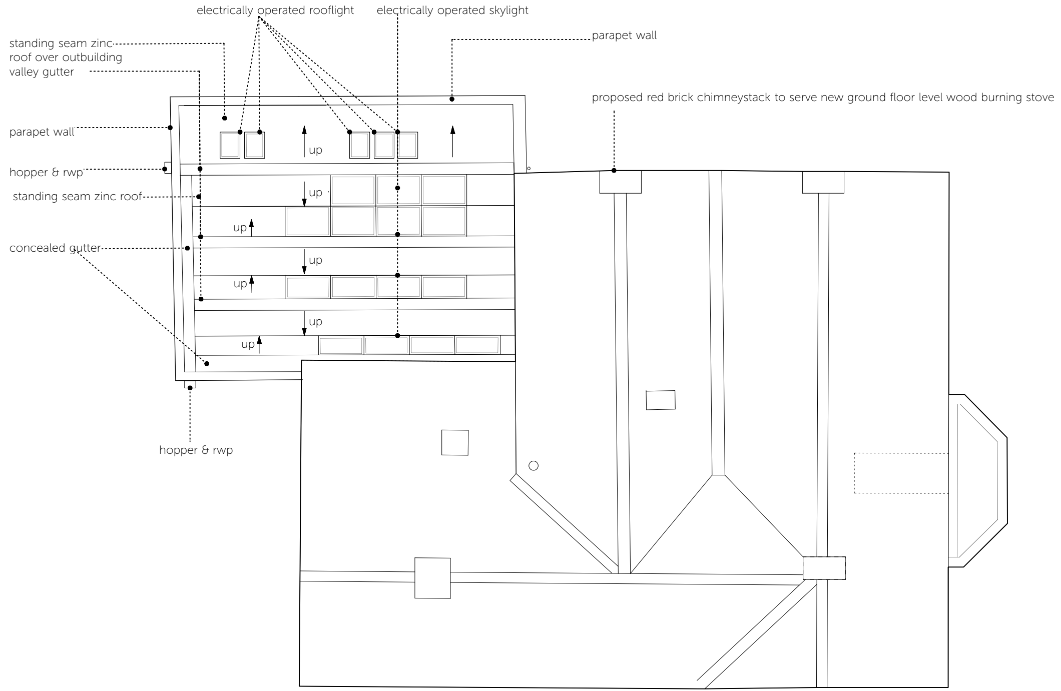
1 Proposed Roof Plan Scale: 1:100
