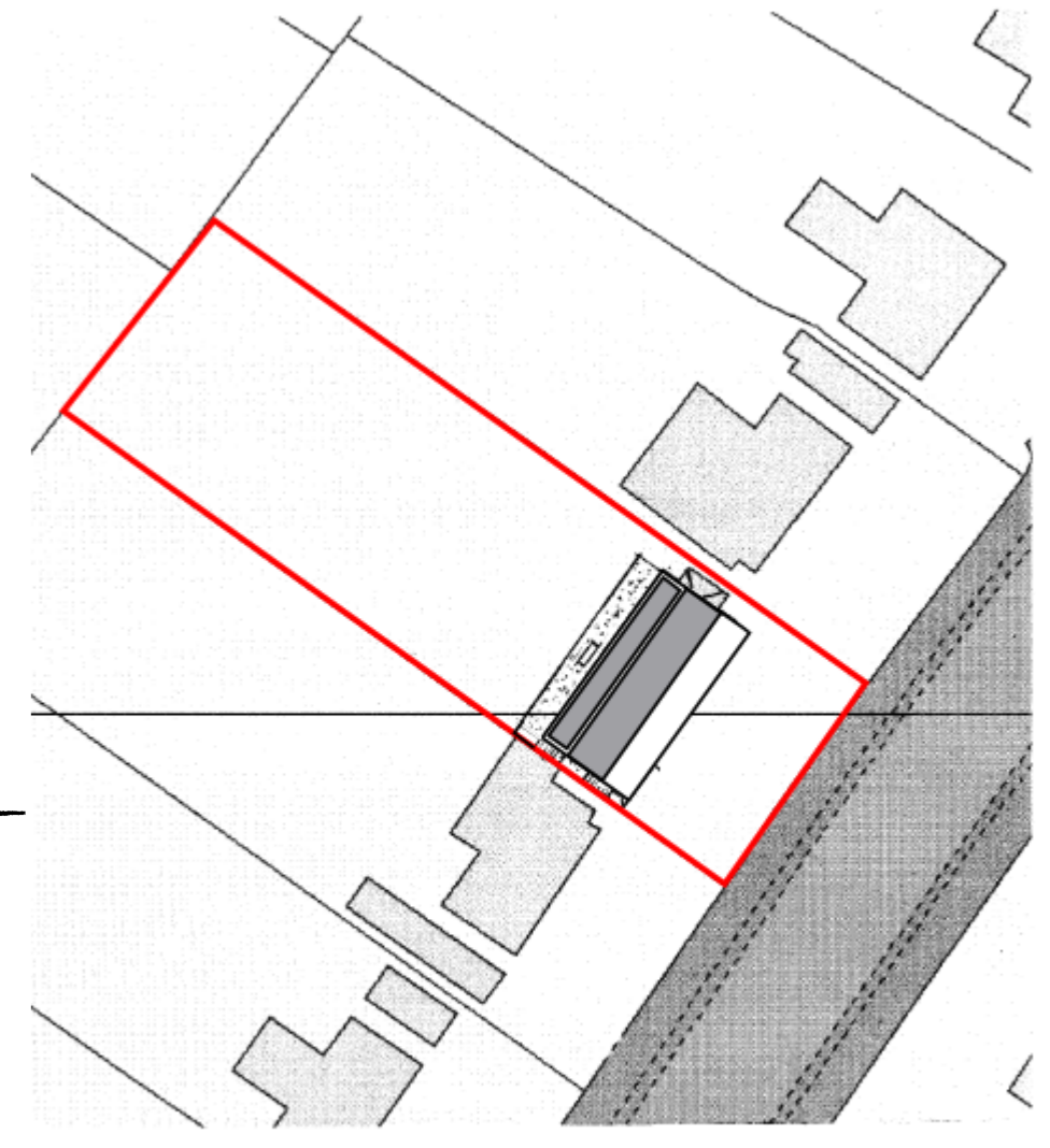
ROOF & BLOCK PLAN @ 1:500
