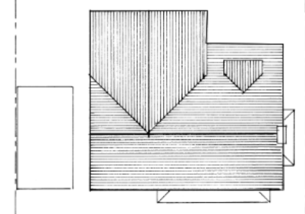
EXISTING ROOF PLAN @ 1:200
