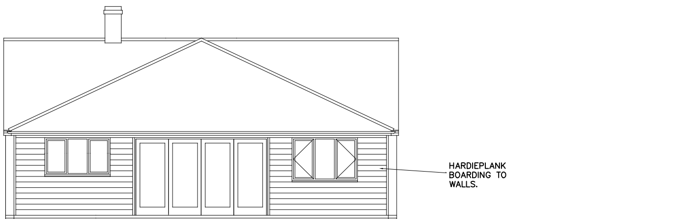
REAR ELEVATION
