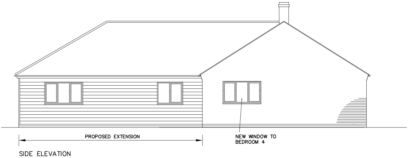
SIDE ELEVATION
