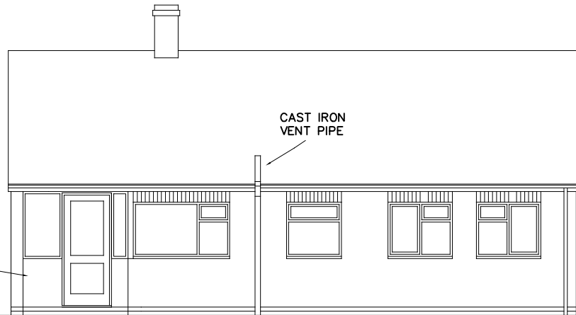
REAR ELEVATION
