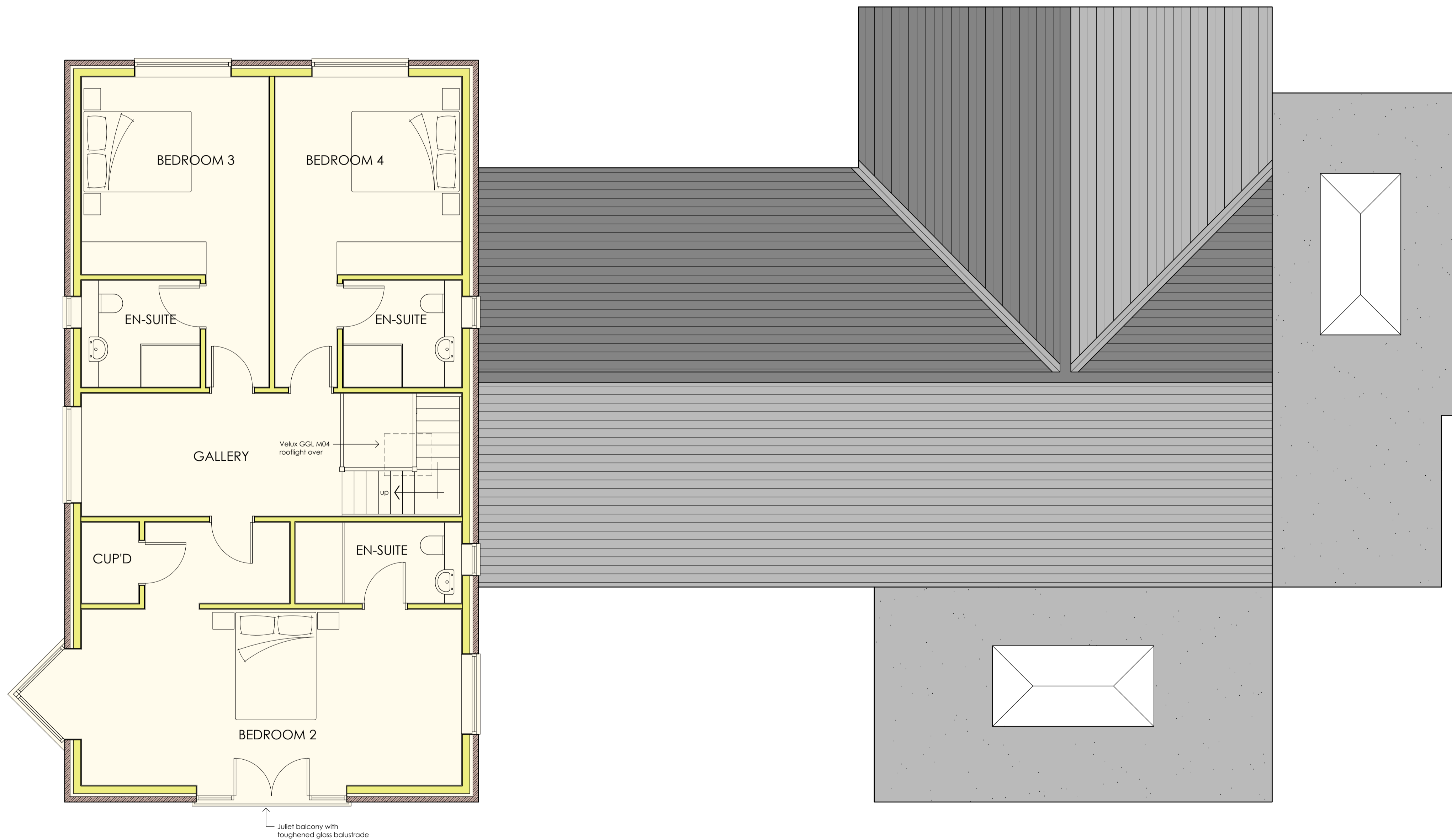
PROPOSED FIRST FLOOR PLAN SCALE 1:50
