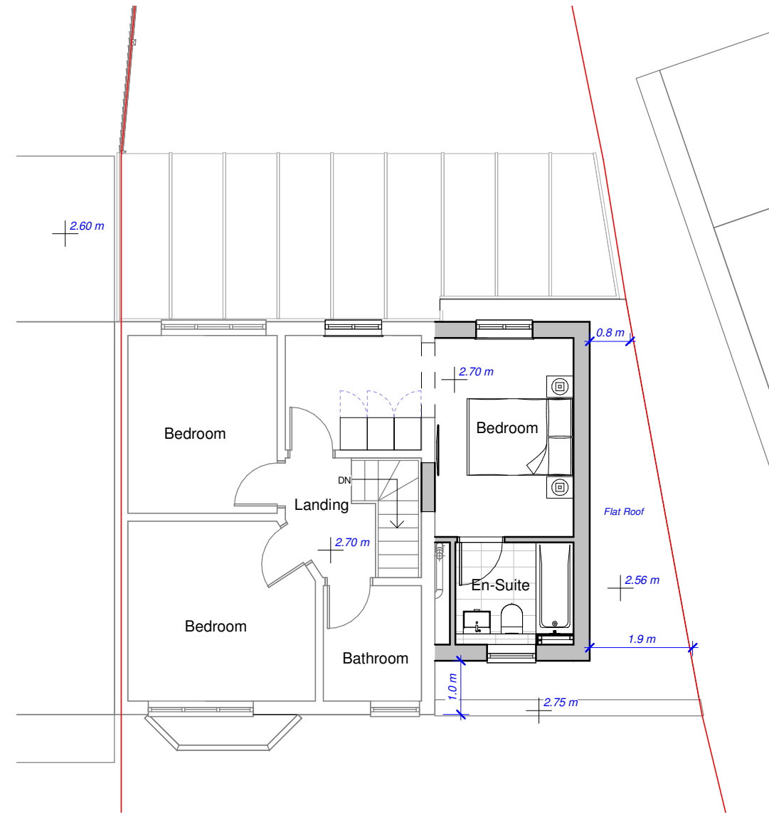
2 First Floor 1 : 100
