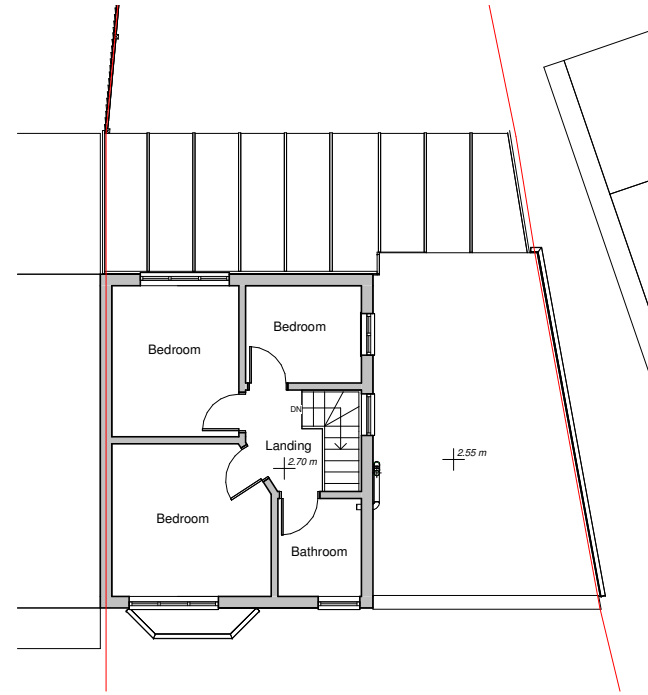
2 First Floor 1 : 100
