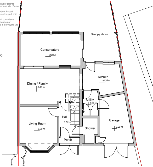
1 Ground Floor 1 : 100
