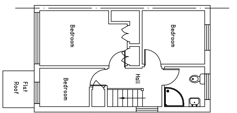
Pre-Existing First Floor Plan @1:100
