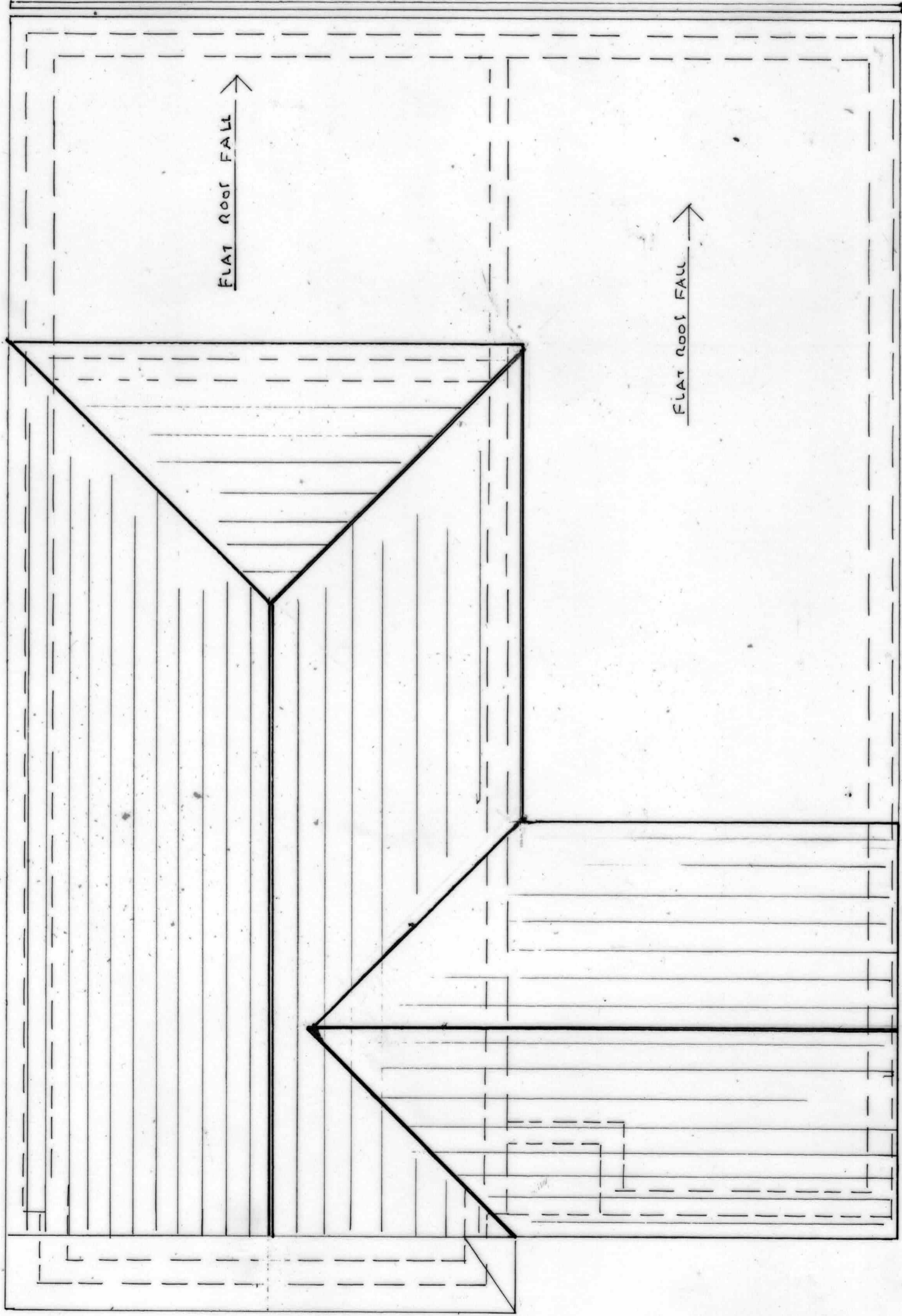
Roof Plan
