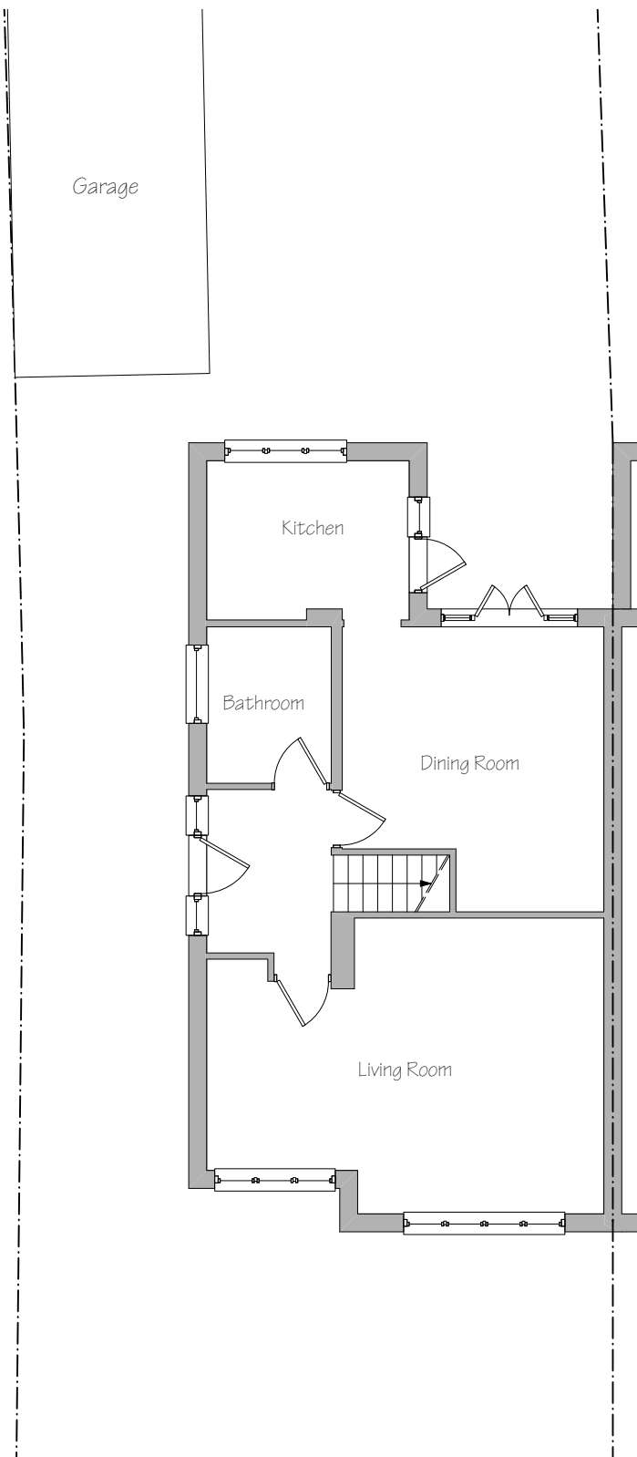
1 Ground Floor
