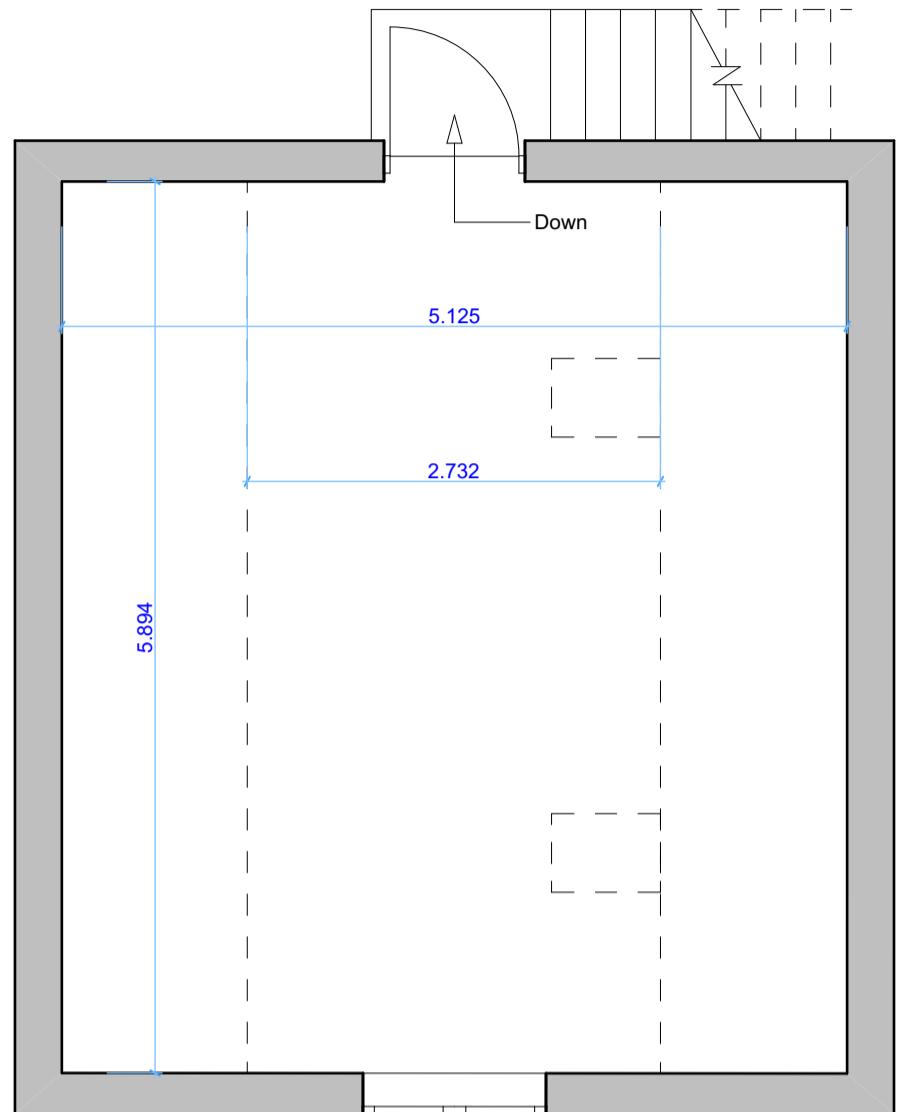
First Floor
