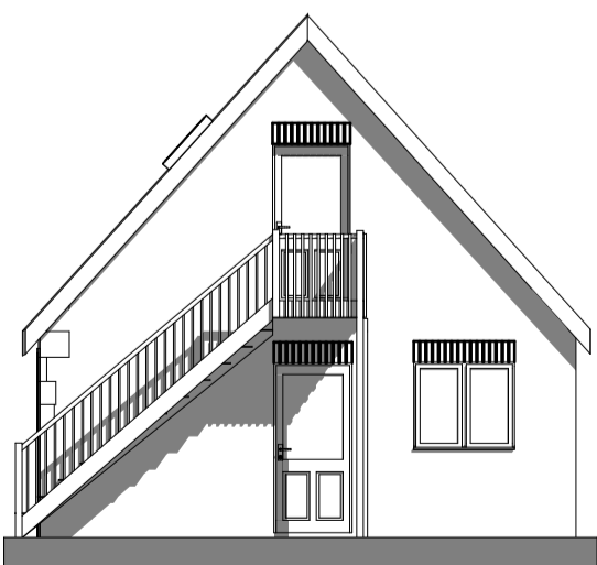
North Elevation 1:100
