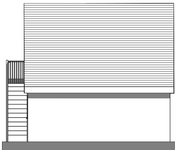
West Elevation 1:100
