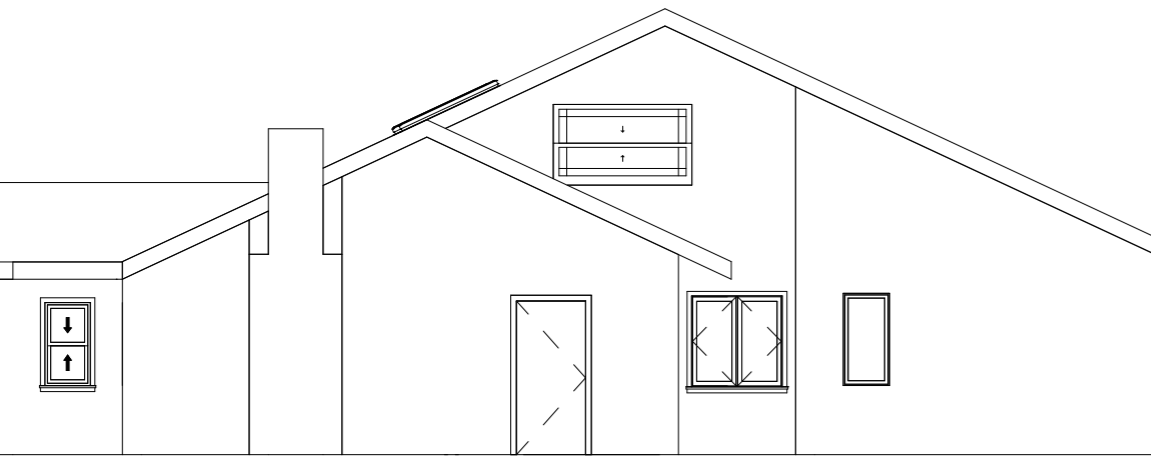
South Elevation
