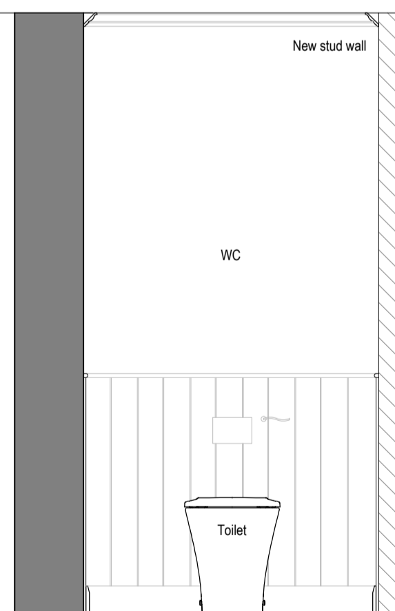
Elevation B Scale 1:20 @ A1
