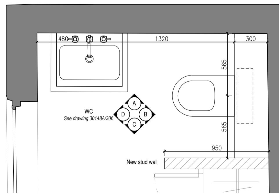
Proposed Ground Floor WC Plan Scale 1:20 @ A1
