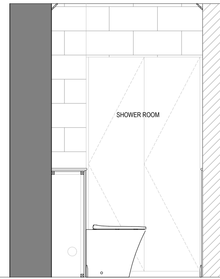
Elevation C Scale 1:20 @ A1
