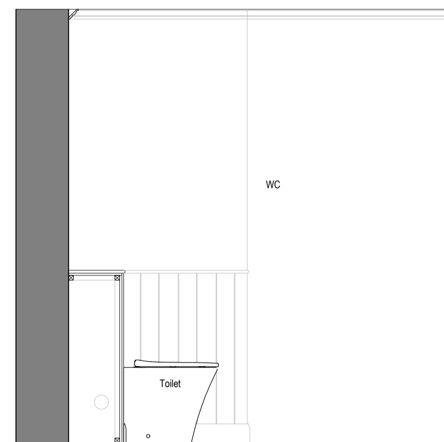
Elevation C Scale 1:20 @ A1
