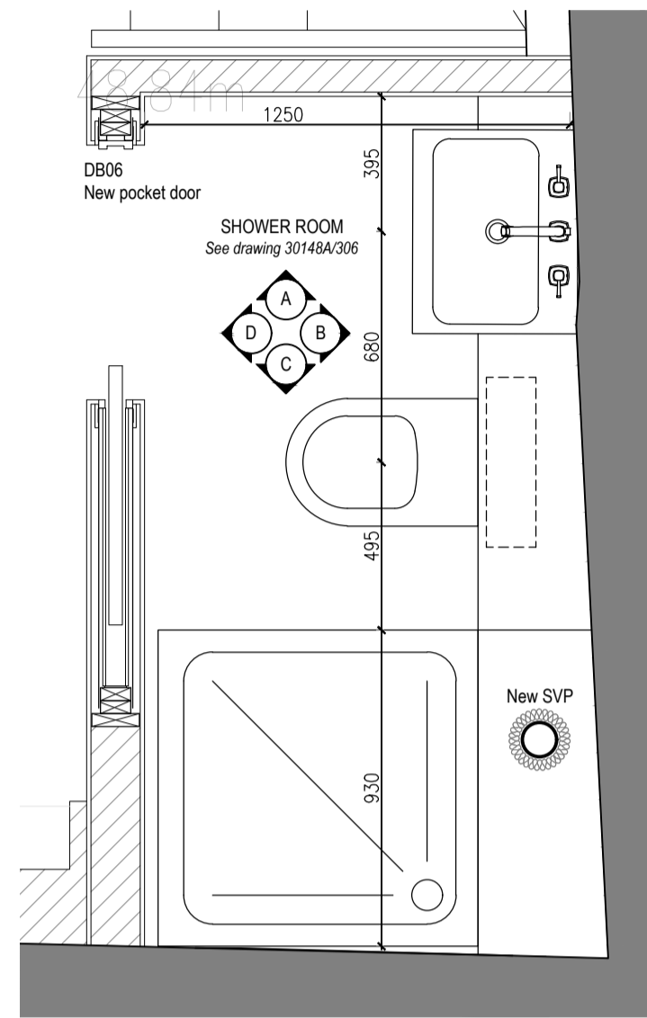
Proposed Basement WC Plan Scale 1:20 @ A1
