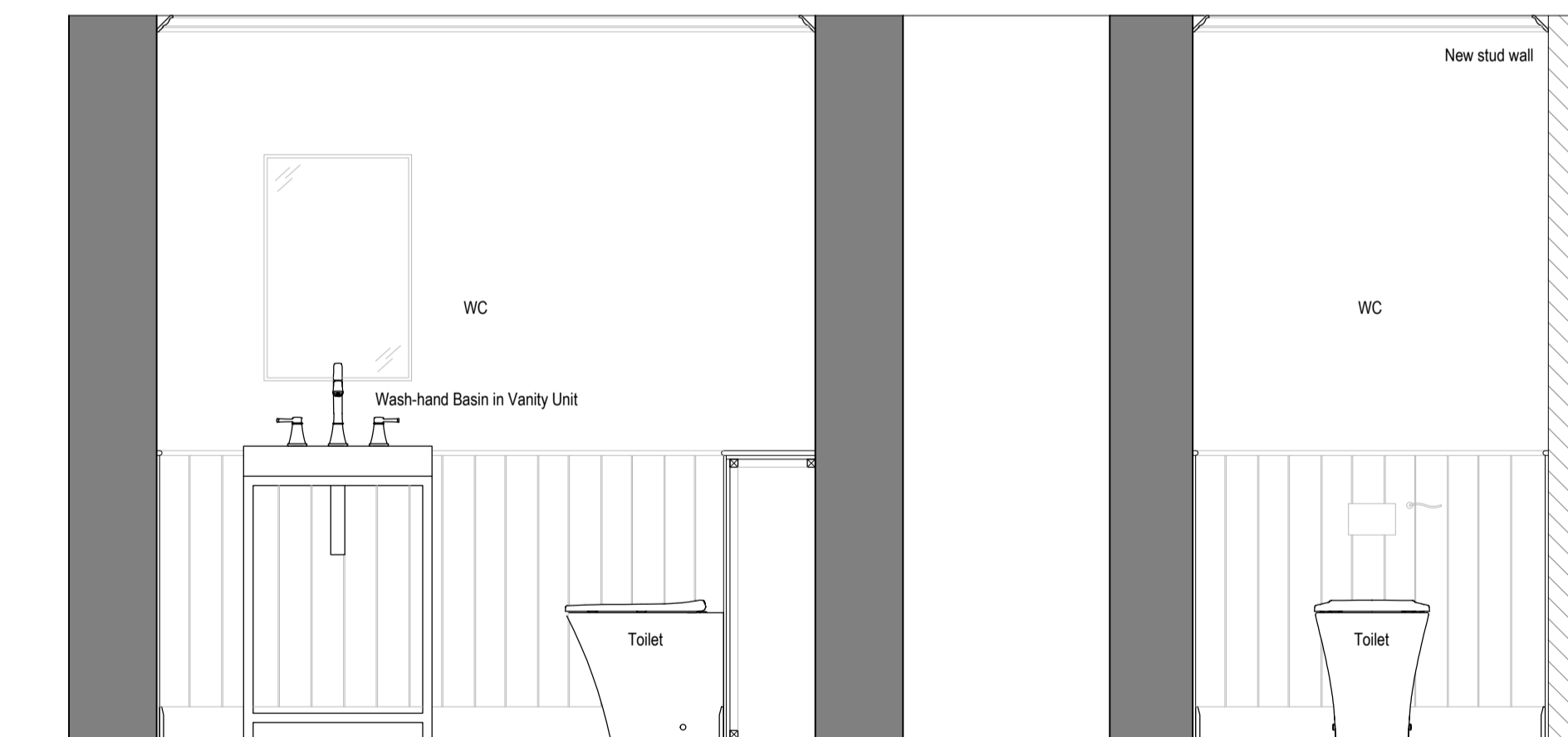
Elevation A Scale 1:20 @ A1
