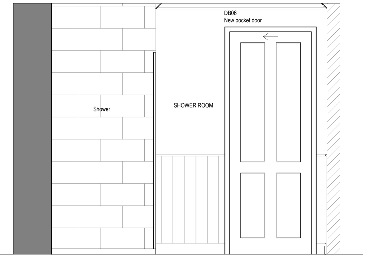
Elevation D Scale 1:20 @ A1
