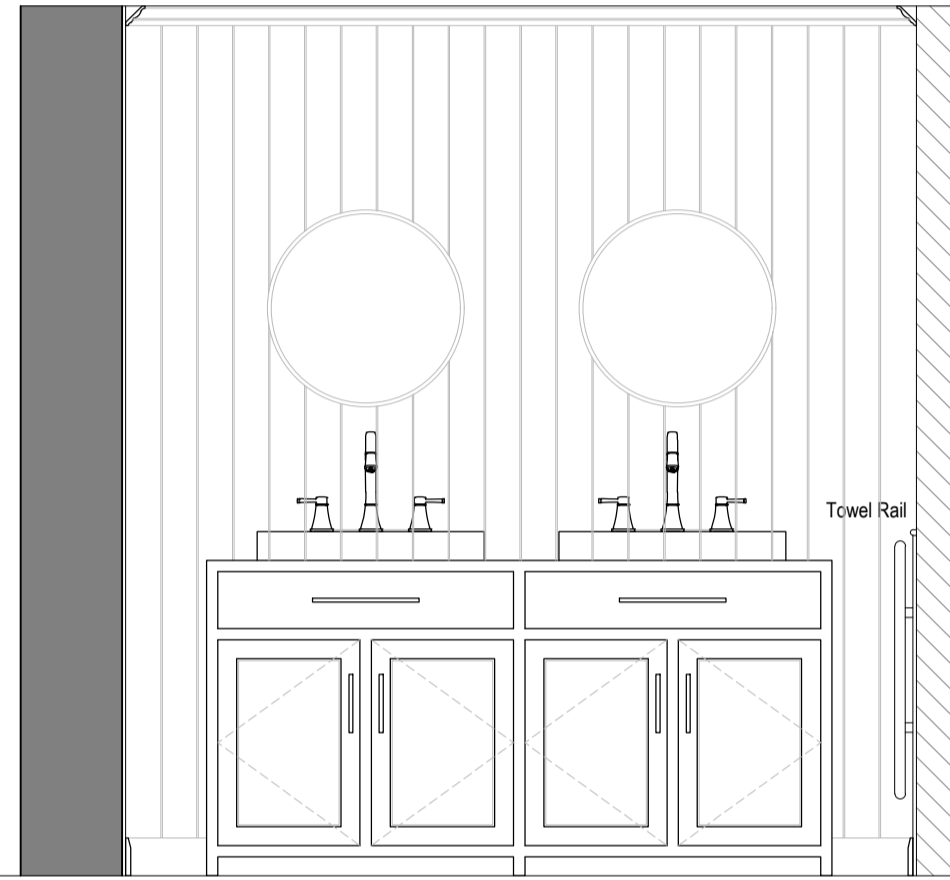
Elevation B Scale 1:20 @ A1
