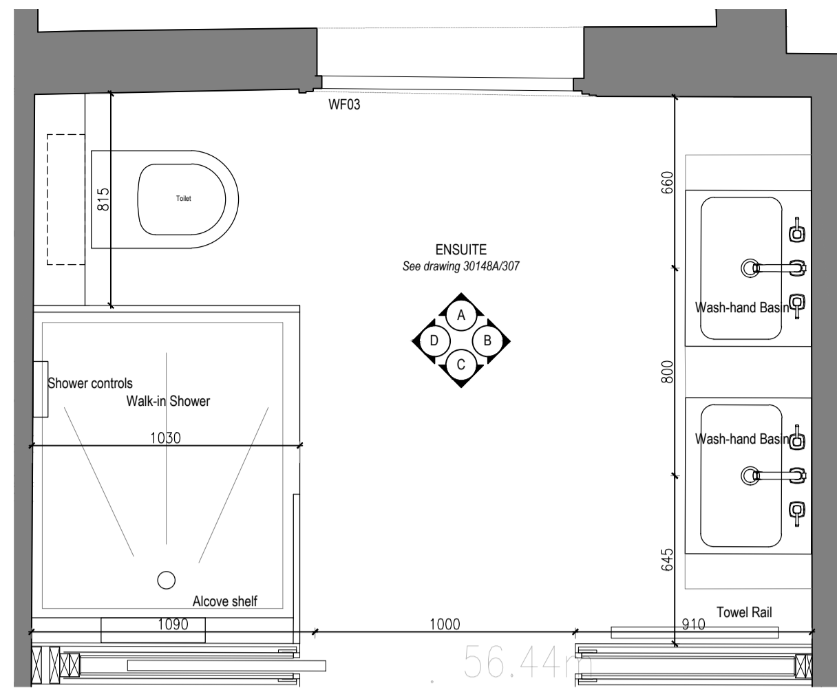
Proposed First Floor Ensuite Plan Scale 1:20 @ A1
