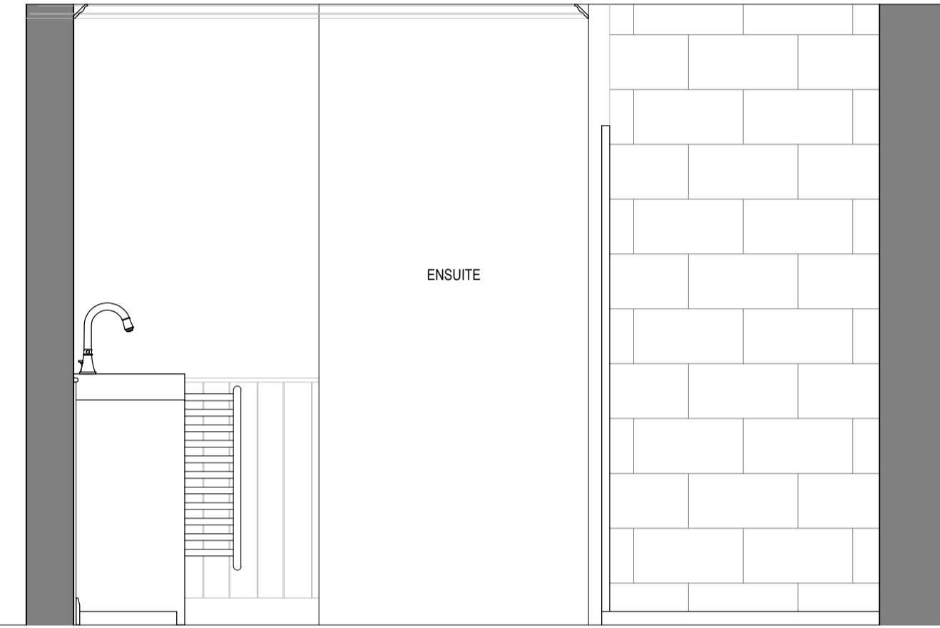
Elevation C Scale 1:20 @ A1
