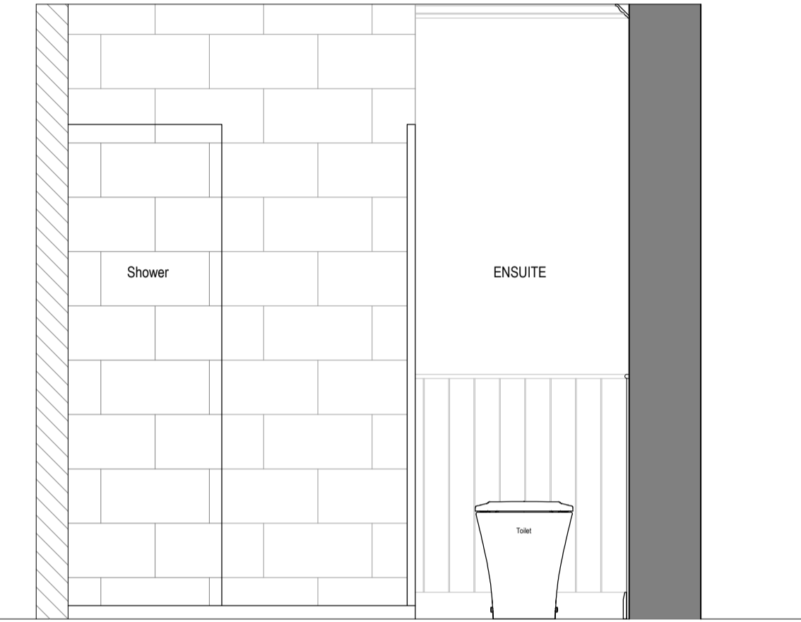
Elevation D Scale 1:20 @ A1
