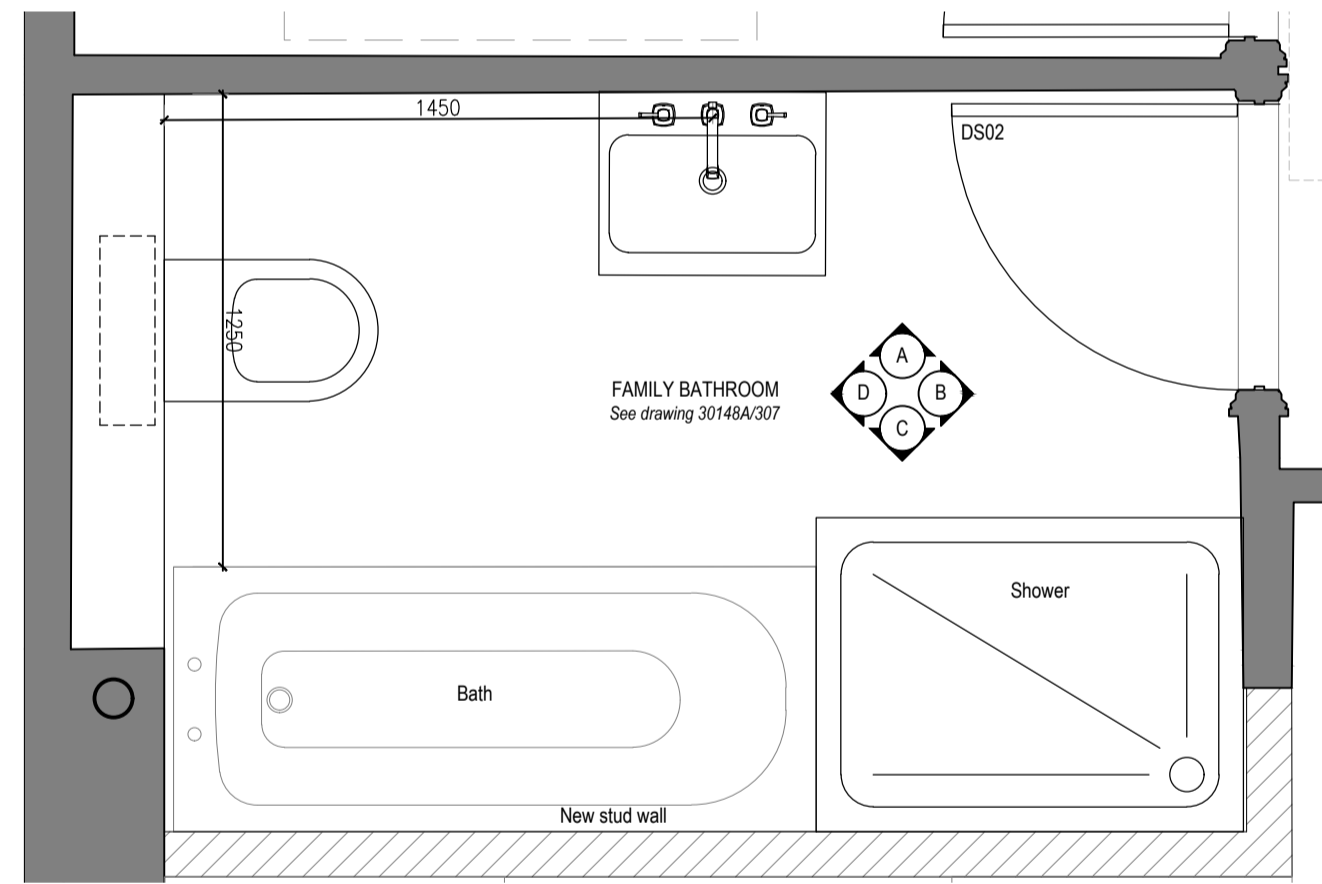
Proposed Second Floor Bathroom Plan Scale 1:20 @ A1
