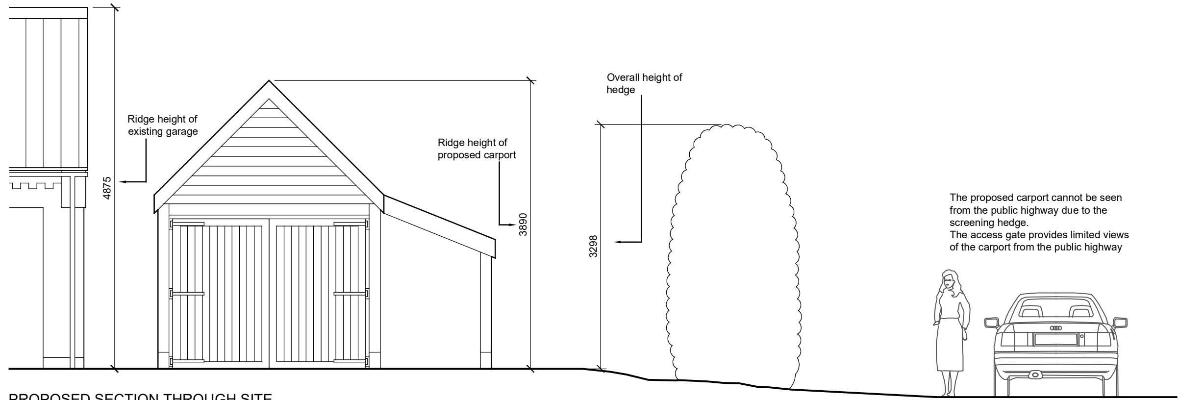
PROPOSED SECTION THROUGH SITE 1:50
