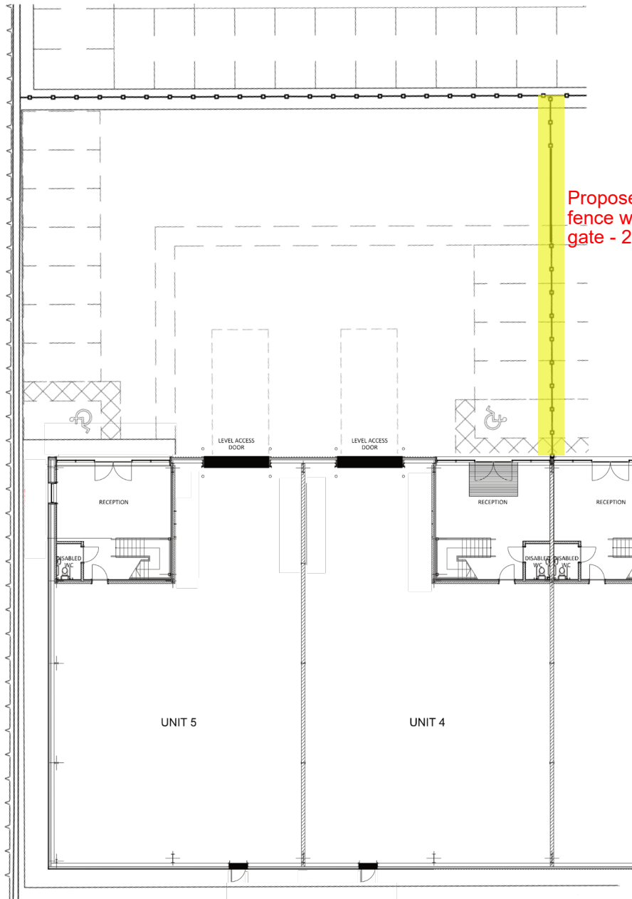
Ground Floor
