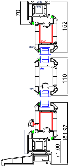
Single door, Open In standard upvc threshold cill
