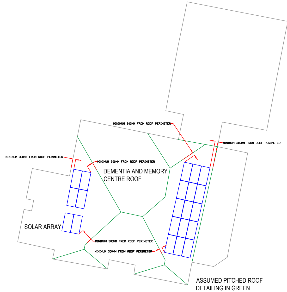
PLAN VIEW
