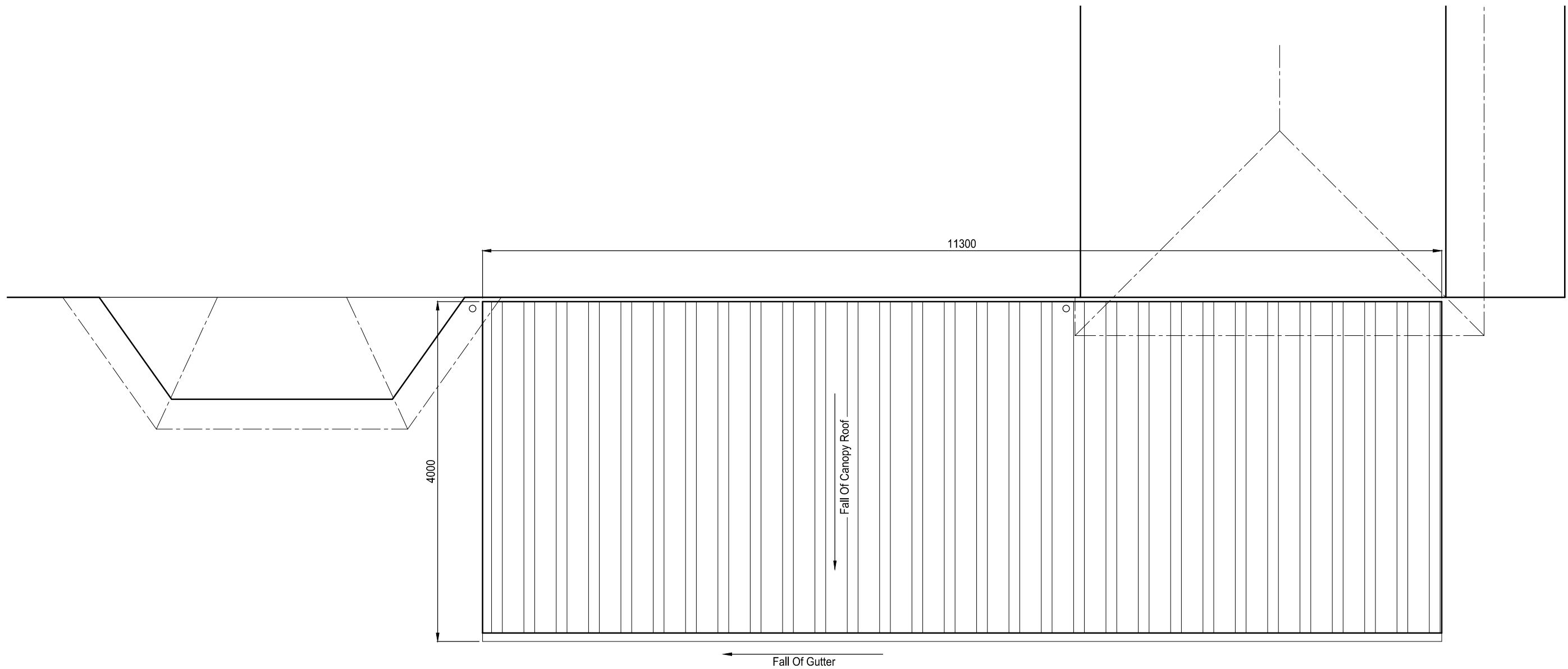
Plan On Canopy Roof Scale 1:50
