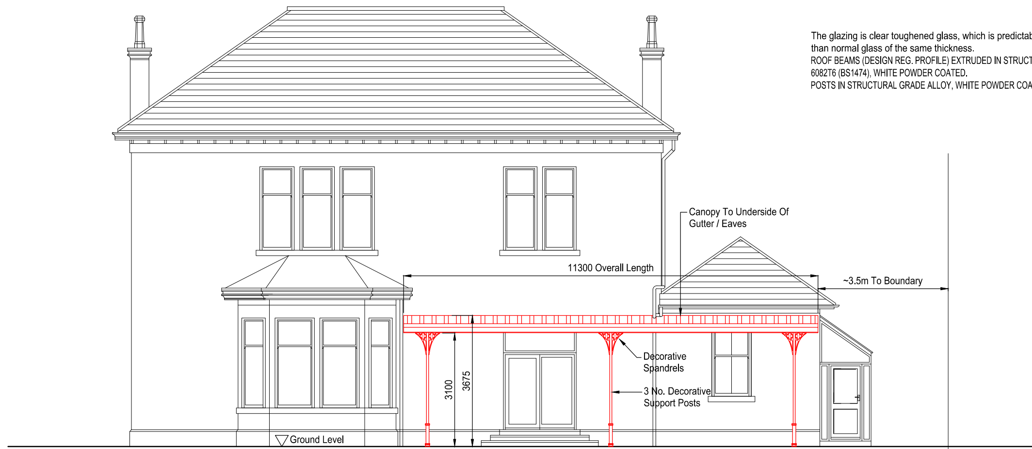
Proposed South Elevation Scale 1:100
