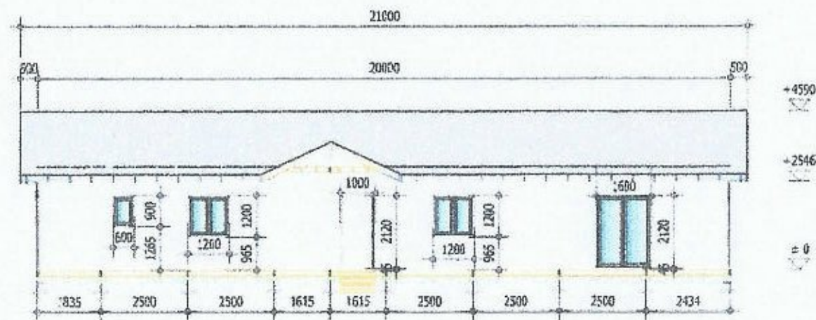
North Elevation. 1:150
