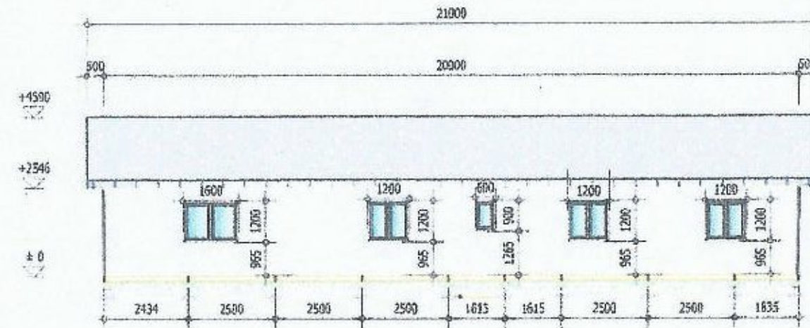
South Elevation. 1:150
