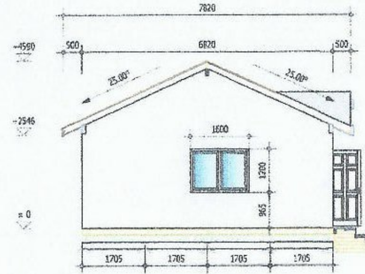
East Elevation. 1:100
