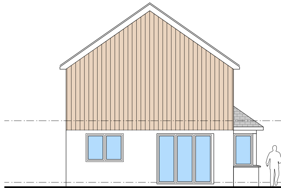
WEST ELEVATION
