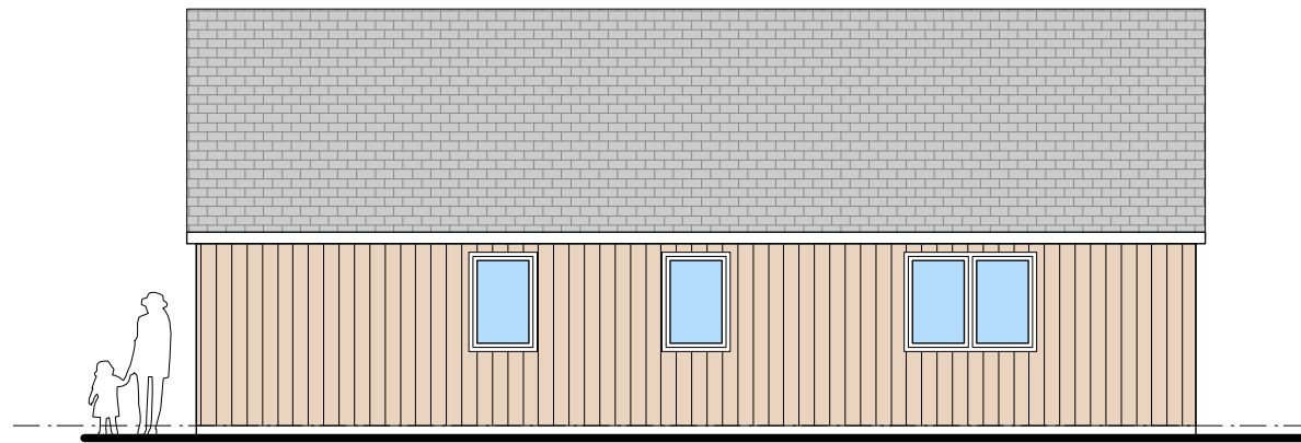
NORTH ELEVATION
