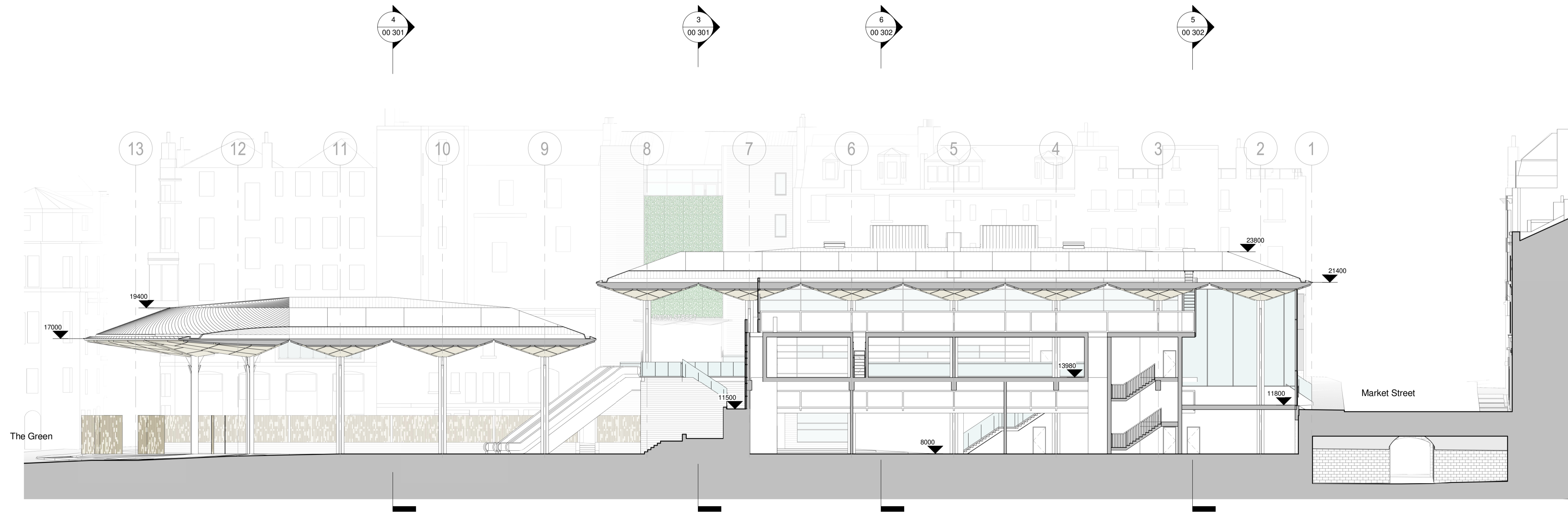
2 General Arrangement Section 2 1 : 200
