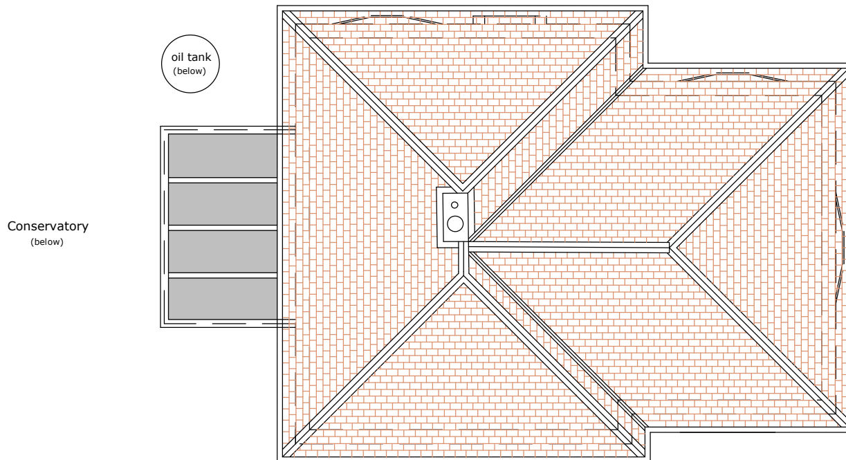
0 Existing Roof Plan
