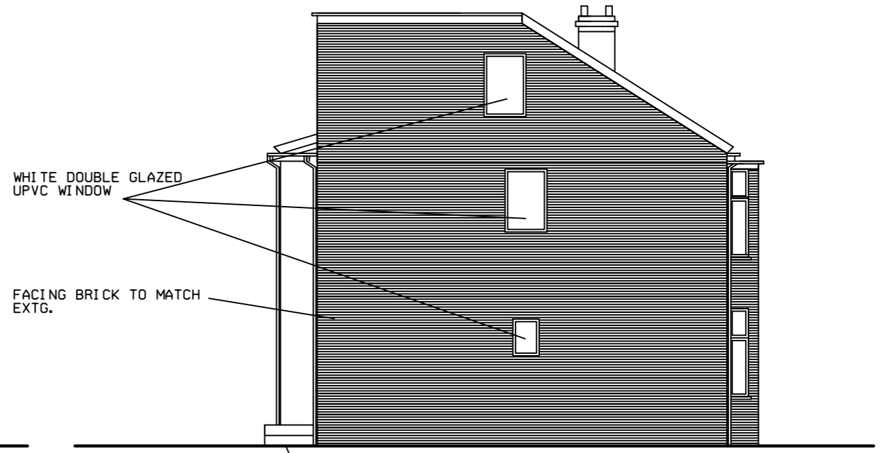
WEST ELEVATION
