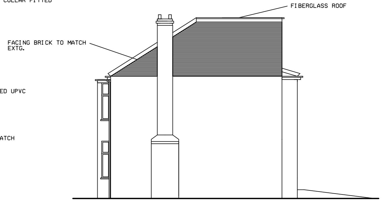
EAST ELEVATION
