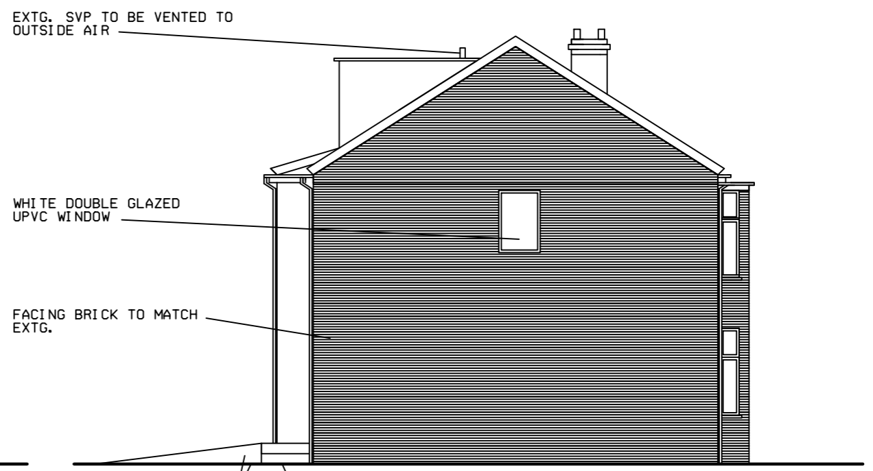
WEST ELEVATION
