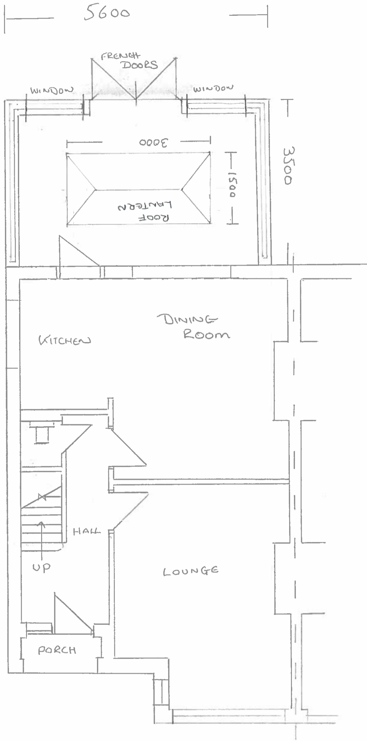
1:50 GROUND FLOOR PLAN
