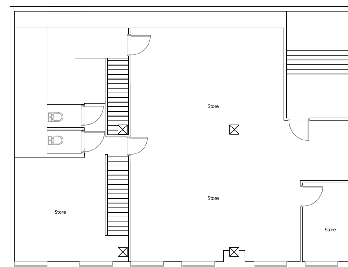
PROPOSED FIRST FLOOR-OPT 01
