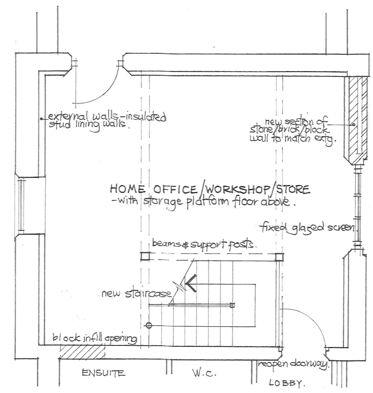
GROUND FLOOR PLAN - AS PROPOSED 1:50
