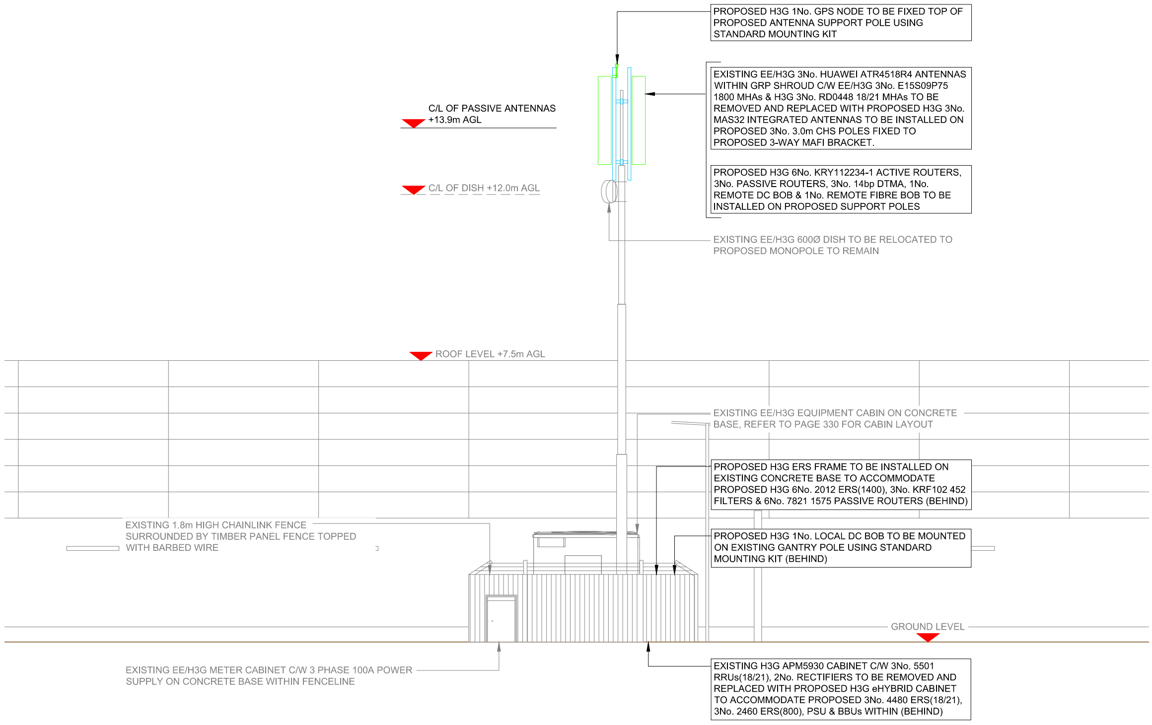
Proposed H3G Site Elevation
