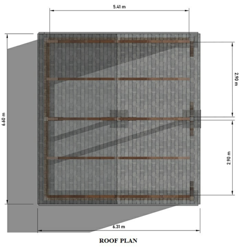
ROOF PLAN
