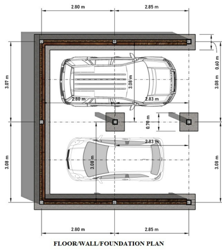
FLOOR/WALL/FOUNDATION PLAN
