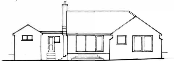
SOUTH EAST ELEVATION
