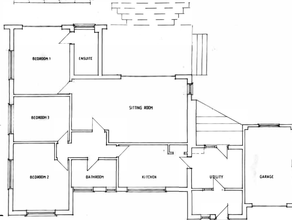
FLOOR PLAN
