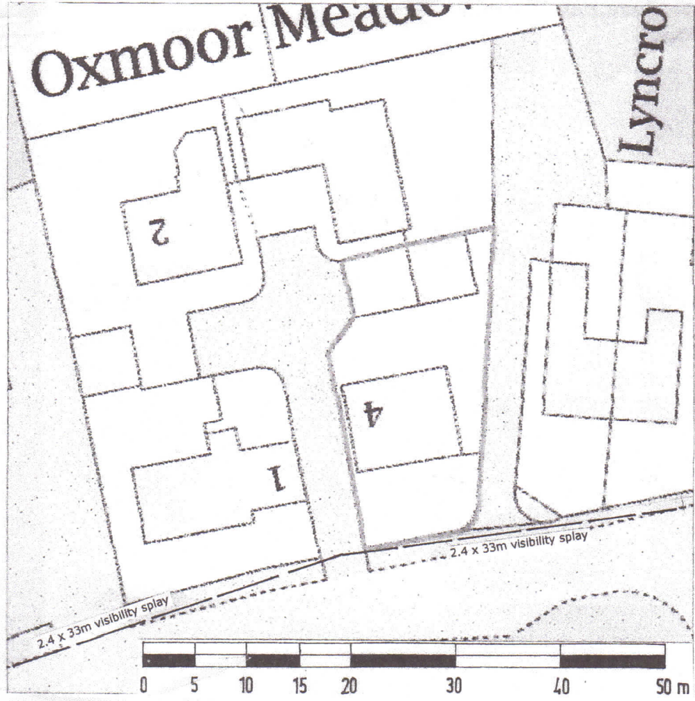
BLOCK PLAN 1:500
