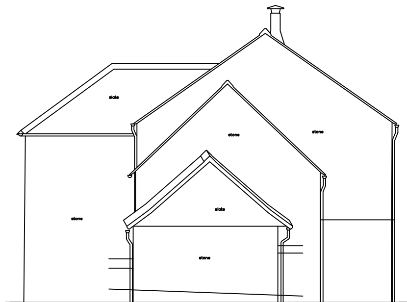
WEST ELEVATION
