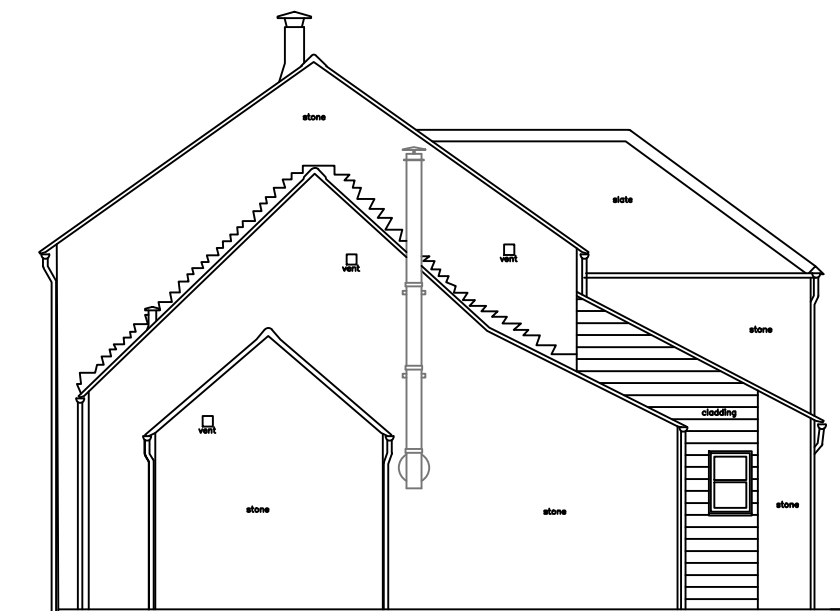
EAST ELEVATION
