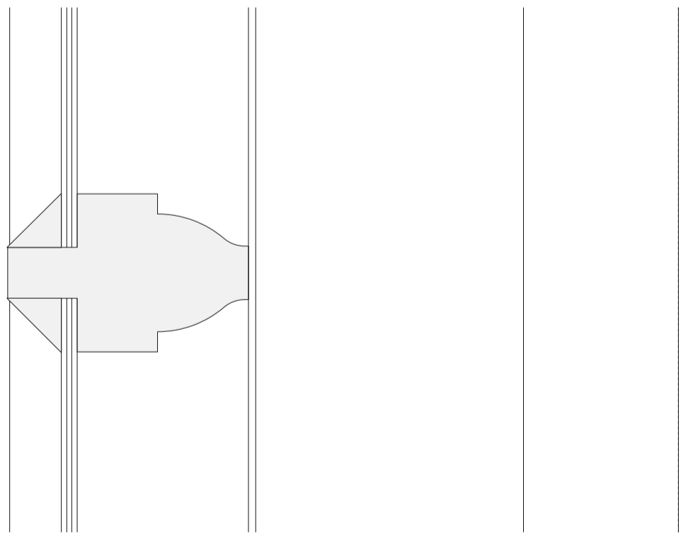
DETAIL B - THROUGH GLAZING BAR
